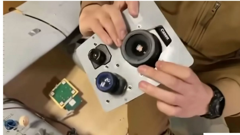
The Canon DSLR camera mounted to a plate.
